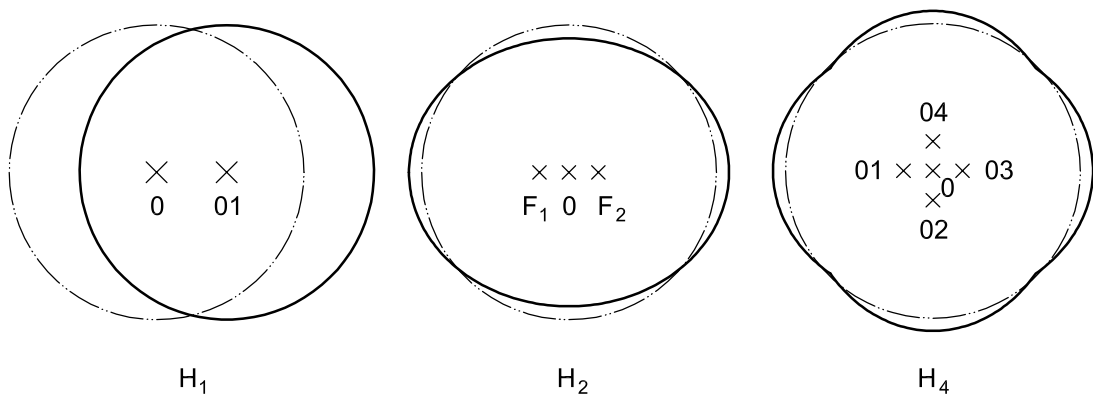
Figure 5 — Geometric representation of the harmonics
