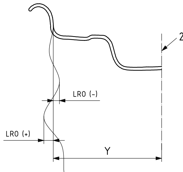
b) Lateral run-out
