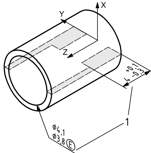
b) Counterbore
