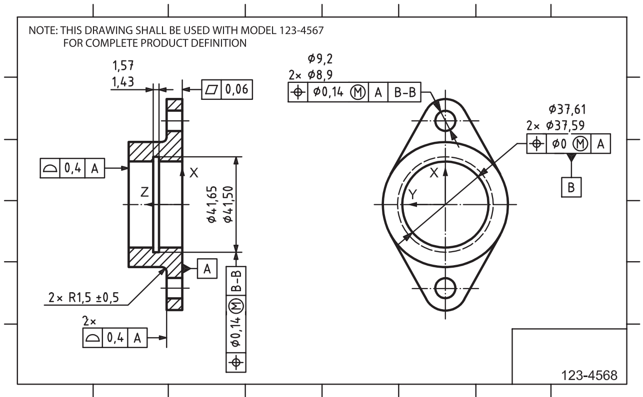
Engineering drawing 123-4568
