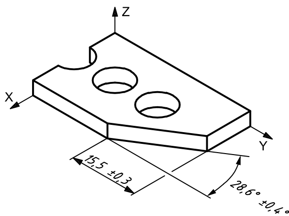
d) Chamfer — Unequal offsets
