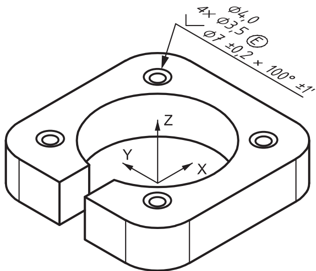
a) Countersinks
