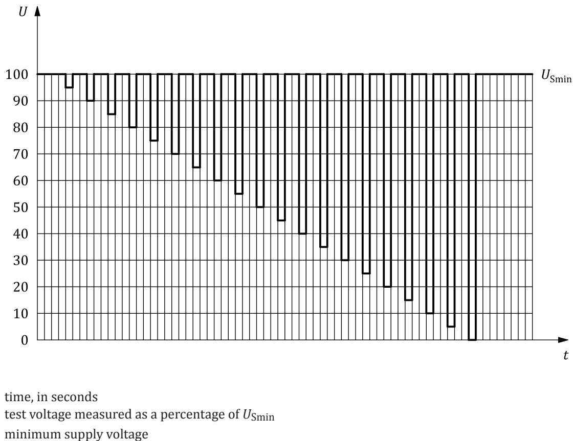
Figure 6 — Supply voltage profile for the reset test
