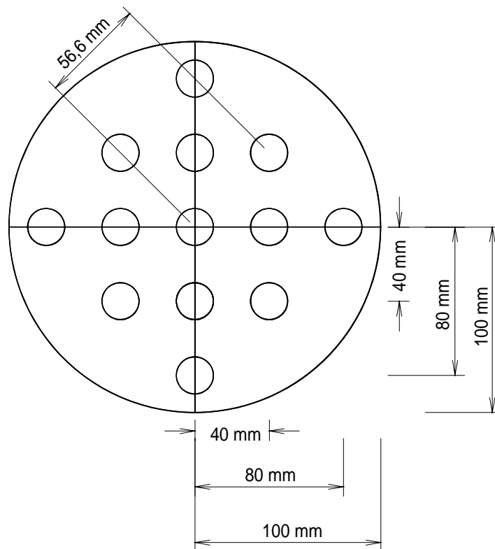
Figure 1 - Location of luminance measurement on roundel signal lights to determine uniformity of luminance.
