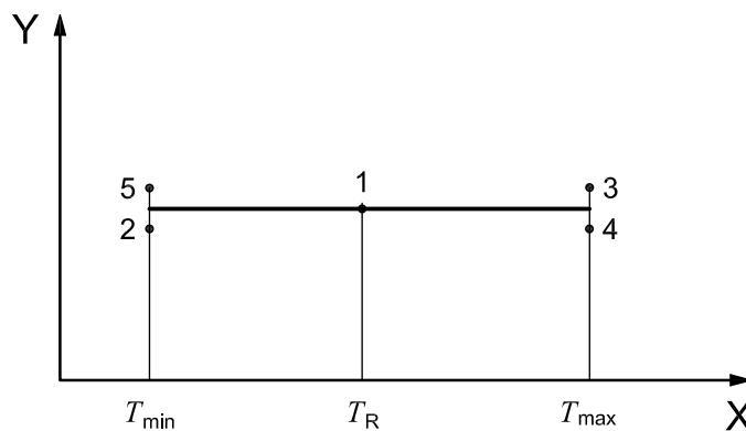
Figure B.2 — Profile with continuous adjustment of energy
