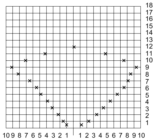
Figure C.2 — Maximum detection points for horizontal plane
