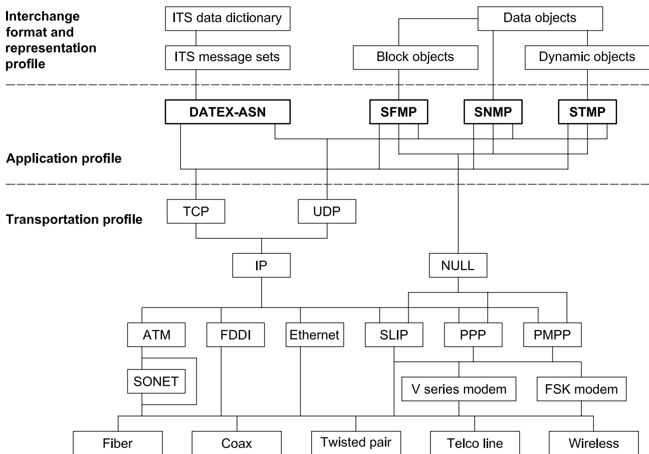
Figure B.1 — Example of protocol stack using multiple application profiles
