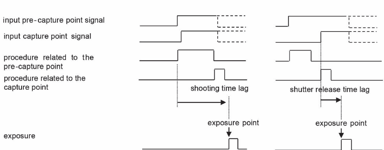
Figure 4 — Measurement period for shooting time lag and shutter release time lag
