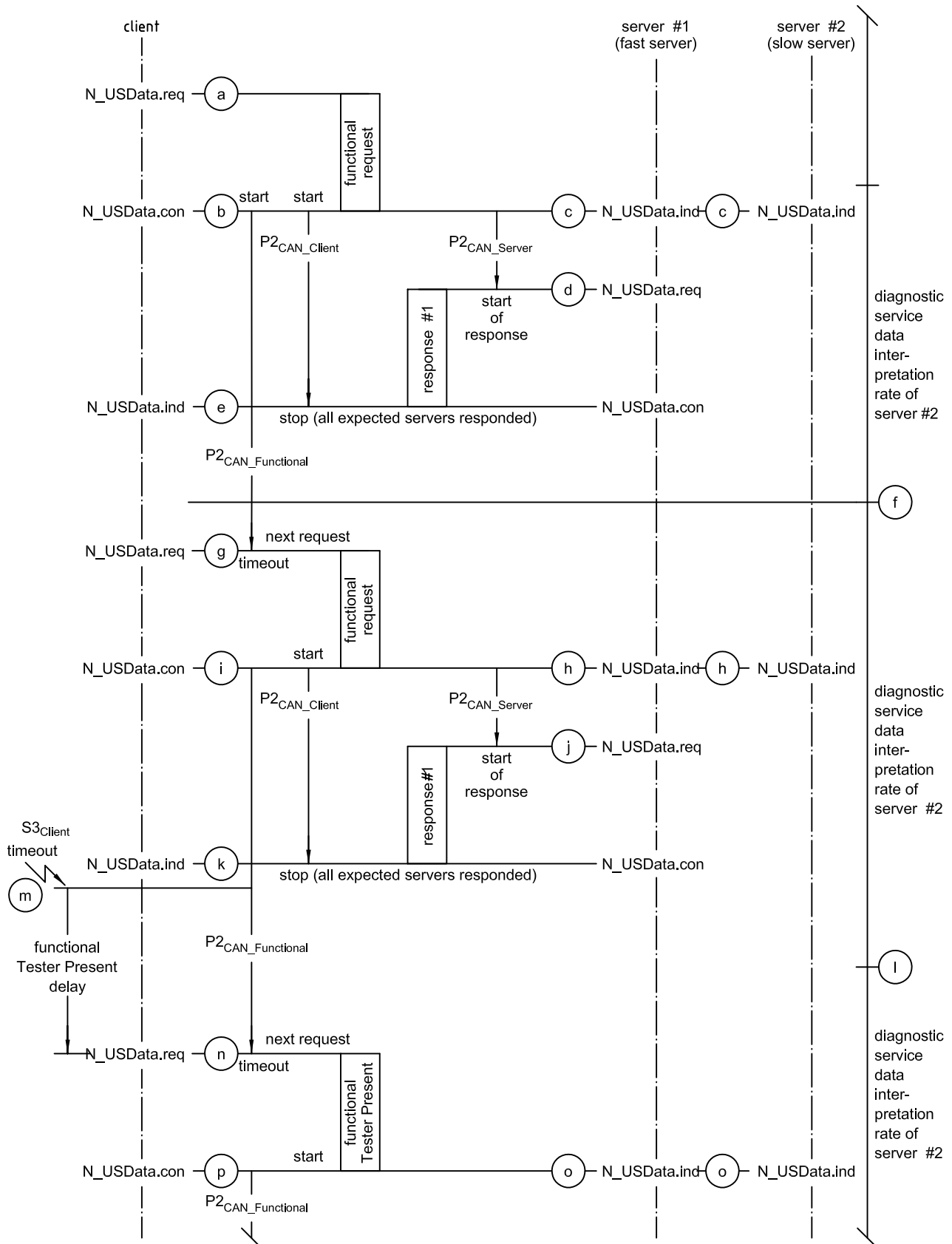
Figure 11 graphically depicts the P3_{CAN\_Functional} timing handling for the client (based on the communication scenario illustrated by Figure 10). In addition, Figure 11 shows the handling of a functionally addressed TesterPresent (3E hex) request message in the client in the case in which the P3_{CAN\_Functional} timer is still active when S3_{Client} times out (request will be postponed until P3_{CAN\_Functional} times out).
