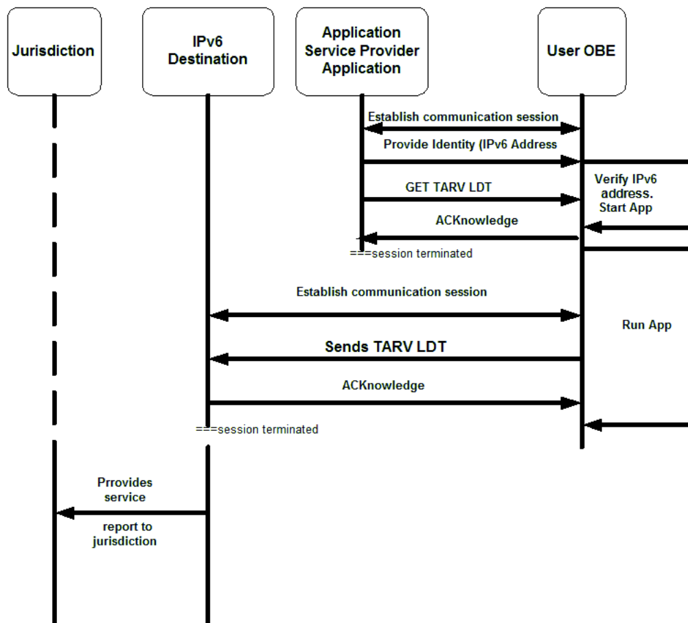
Figure C.1 — Communications sequences to obtain TARV LDT
