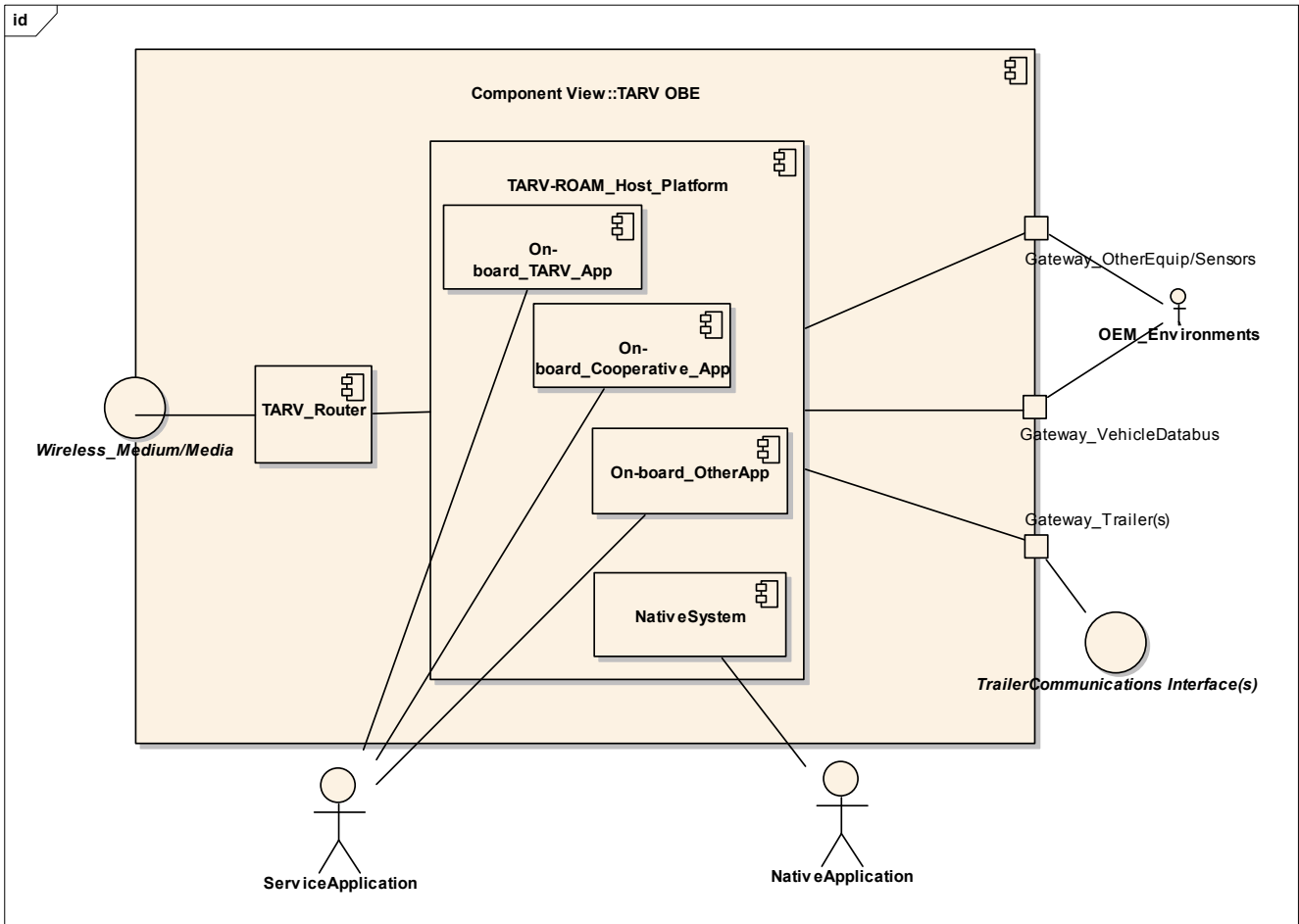
Figure 4 — TARV IVS component decomposition
