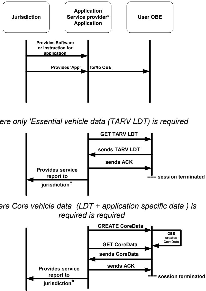
Figure C.2 — Sequences to obtain TARV LDT and CoreData
