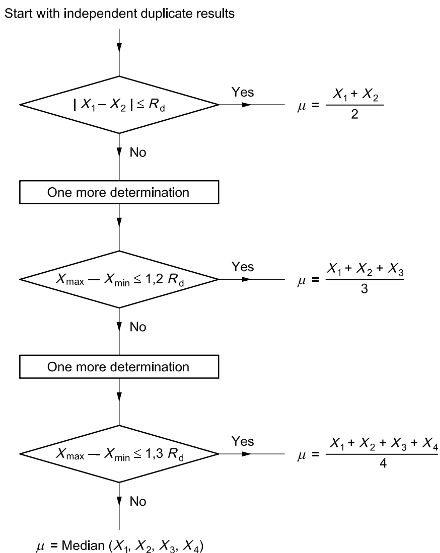
Figure A.1 — Flowsheet
