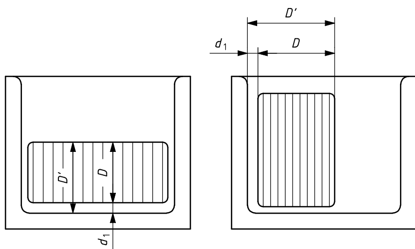
b) Determination of dimensions of fractional shelves
