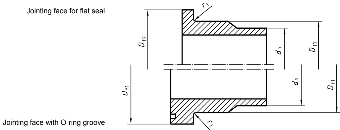
Figure C.8 — Dimensions of flange adaptors for butt fusion
