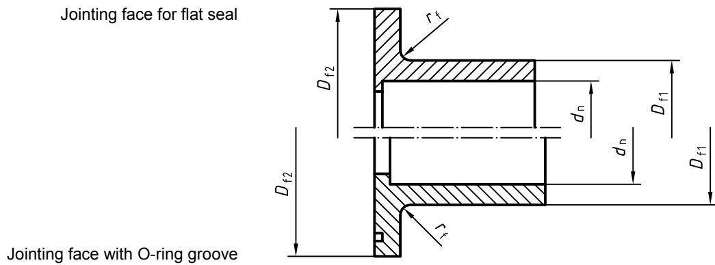
Figure C.10 — Dimensions of flange adaptors for socket fusion
