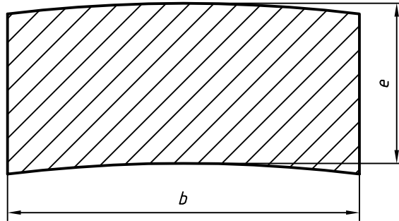
Figure C.12 — Shape of type 2 and type 3 test pieces for impact testing
