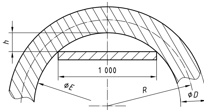
Figure 8 — Coiling of a large diameter hose
