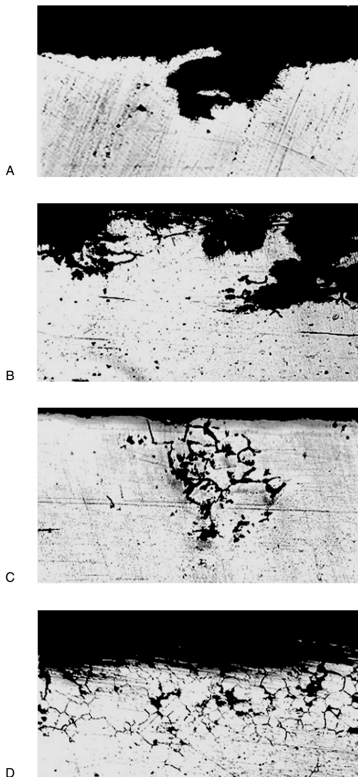
Figure 2 — Types of corrosion showing the aluminium alloy specimens after electrochemical testing
