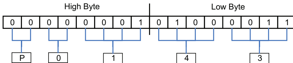
Figure 17 — Diagnostic trouble code encoding example DTC P0143
