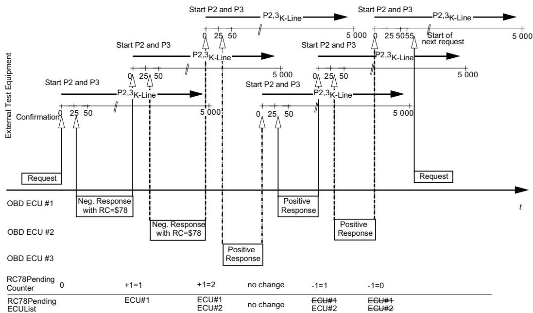
Figure 13 — ISO 14230-4 — Negative response code RC=0x78 handling overview
