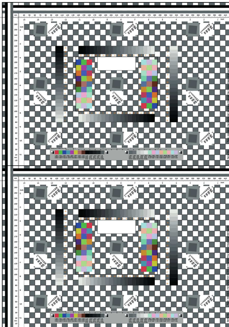
Figure C.2 — A2 arrangement
