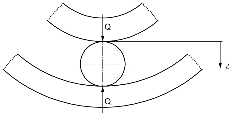
Figure 2 — Total deflection of roller contacts
