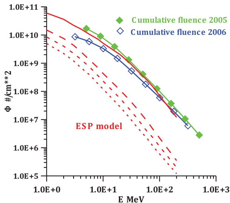
Figure B.1a — ESP model[14] energy spectra predictions for cases of averaged (dotted curve) and worst solar minimum years (short dashed curve)
