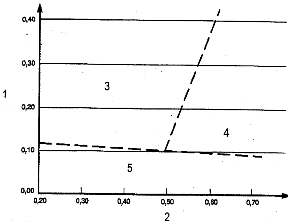
Figure 12 — Critical cooling rate for 350 HV and 400 HV
