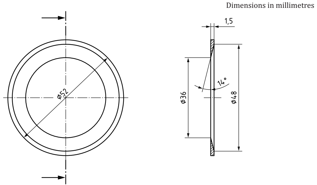
Figure F.4 — Aperture disc
