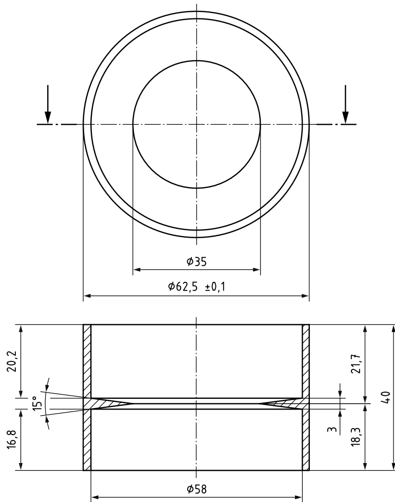
Figure F.5 — Spacer ring
