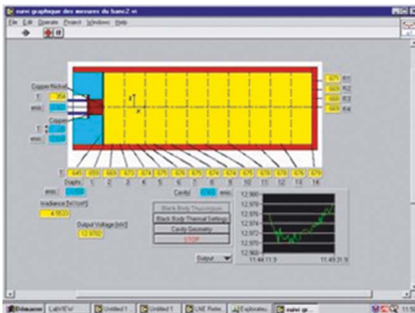
Figure C.1 — Example of temperature gradients along the cavity
