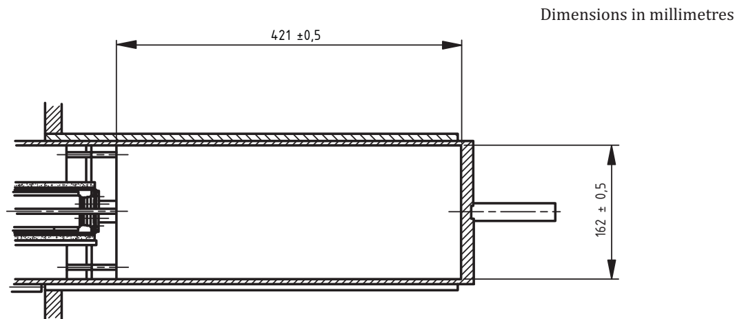
Figure 3 — Cross-section of the black-body cavity
