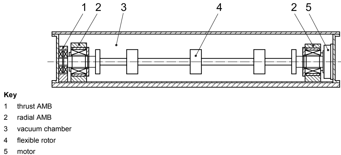
Figure A.1 — Test rig
