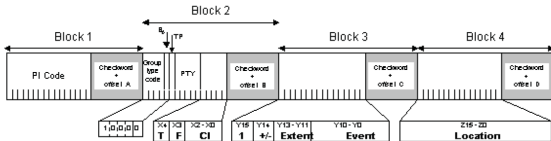
Figure 6 — RDS-TMC multi-group message - first group
