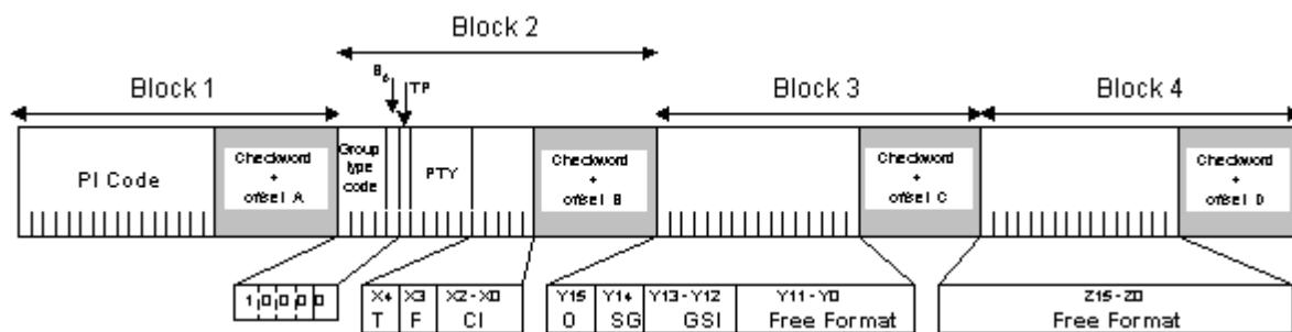
Figure 7 — RDS-TMC multi-group message - subsequent group structure
