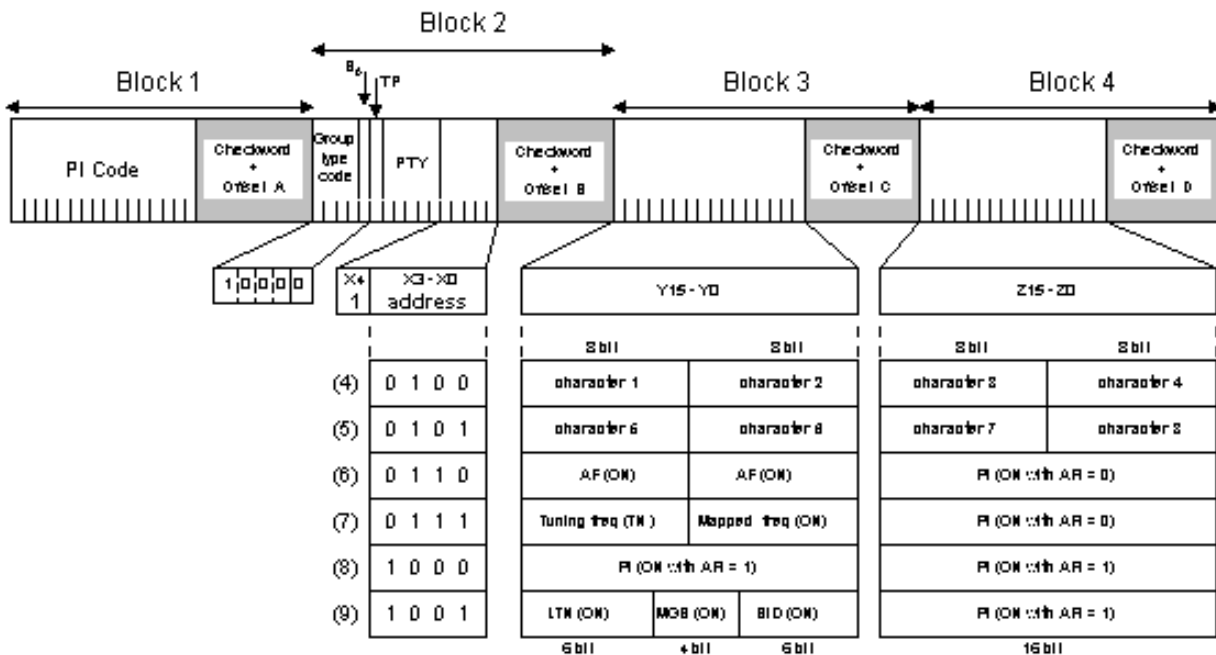
Figure 5 — Format of RDS-TMC tuning information
