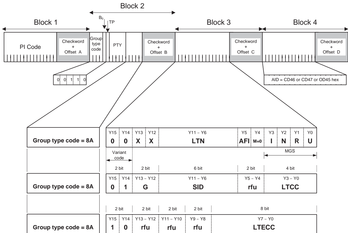
Figure 4 — RDS type 3A group structure, RDS-TMC carrying system information
