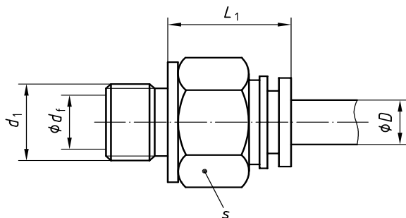
Figure 3 — Stud adaptor (SDS)
