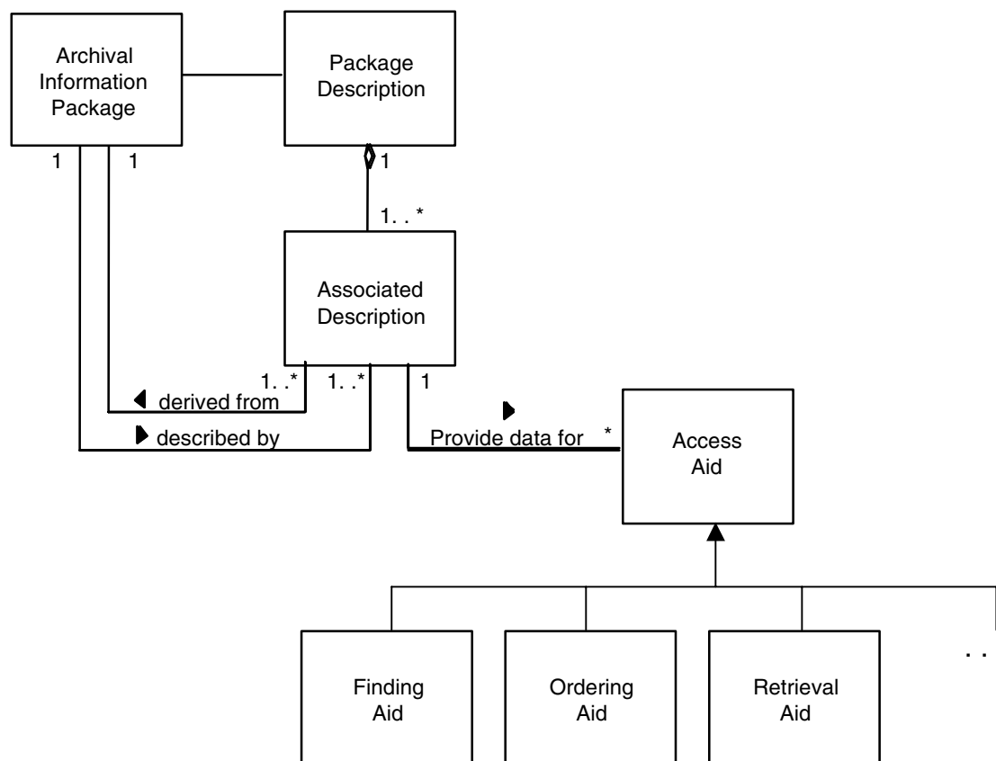
Figure 4-17: Package Description
