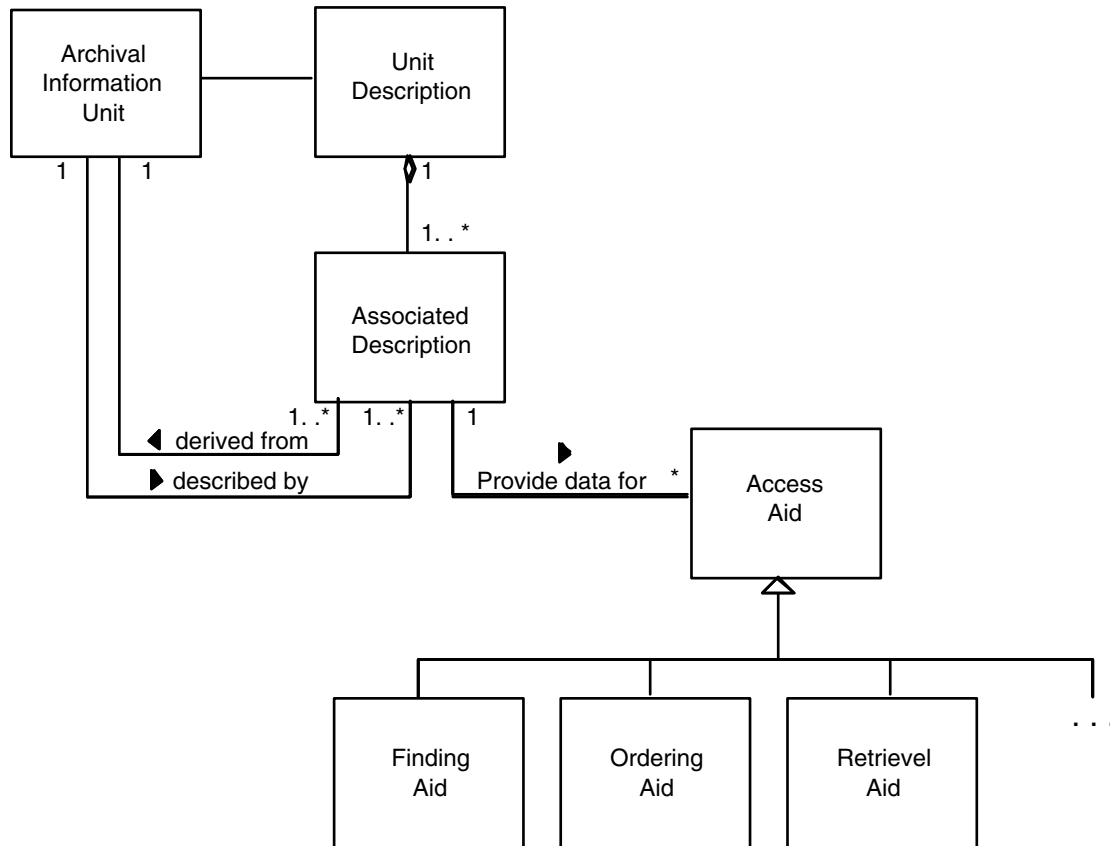
Figure 4-22: Unit Description
