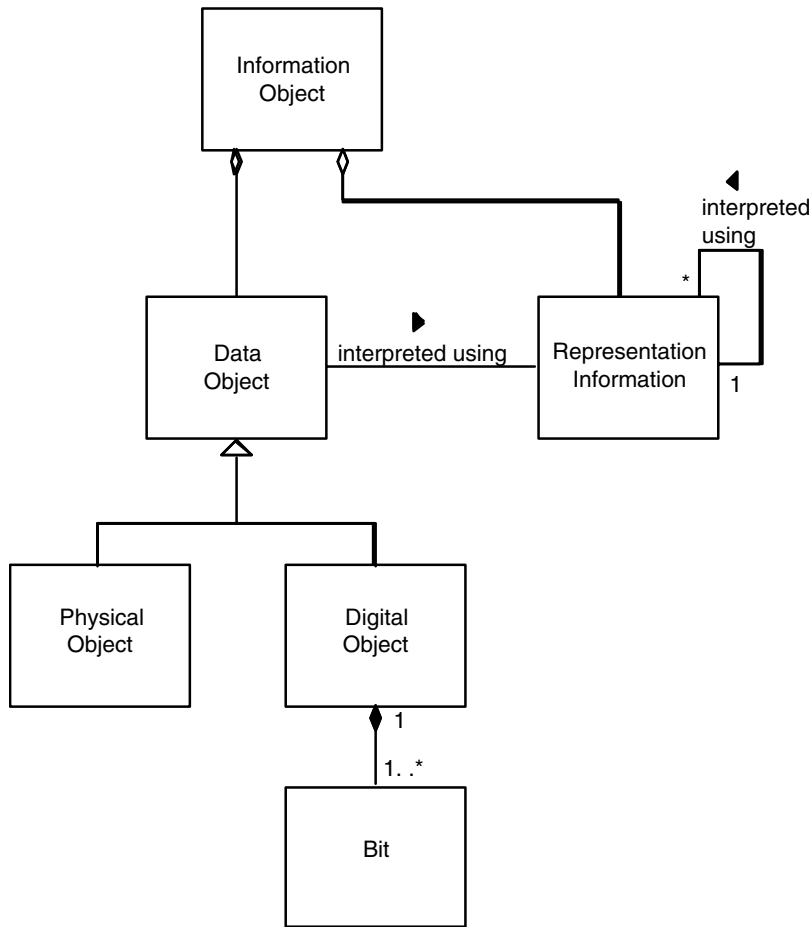
Figure 4-10: Information Object
