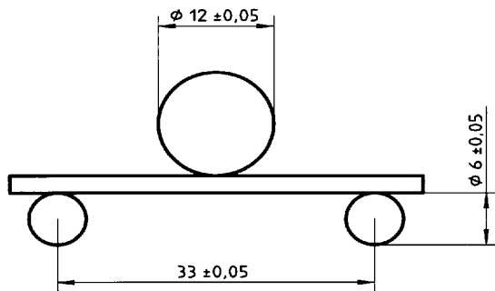
Figure 7 — Test rack
