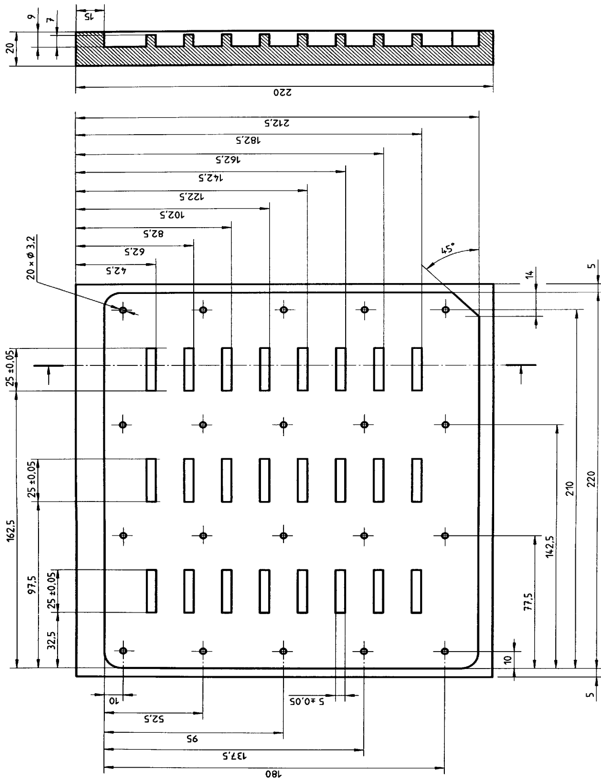
Figure 5 — Silicone rubber mould
