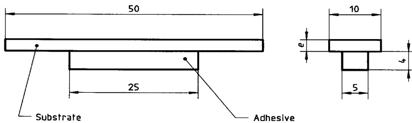
Figure 8 — Specimen
