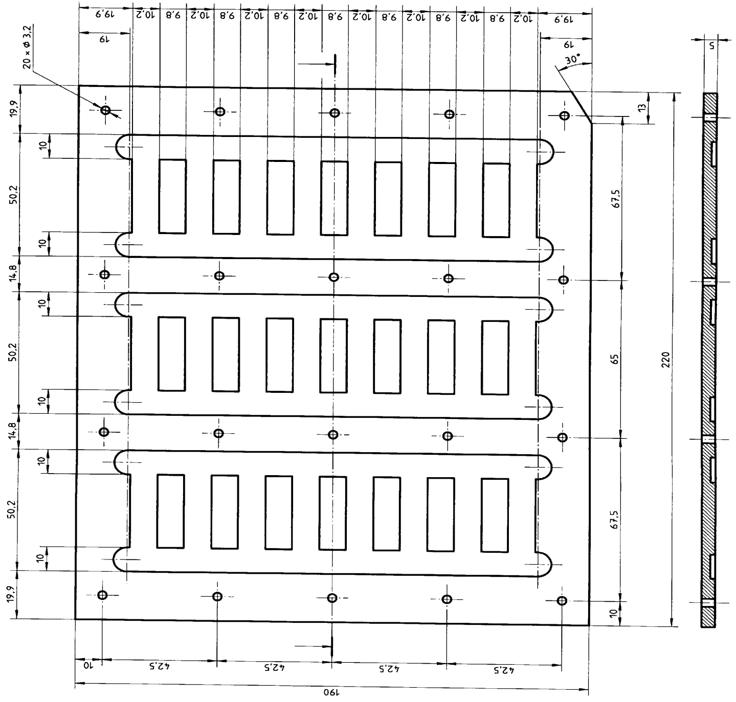
Figure 4 — Lower plate
