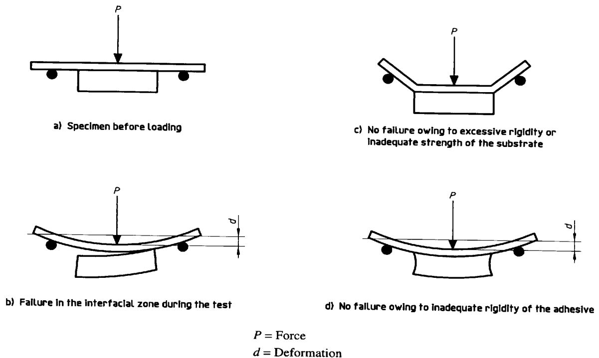
Figure 2 — Principle of the test
