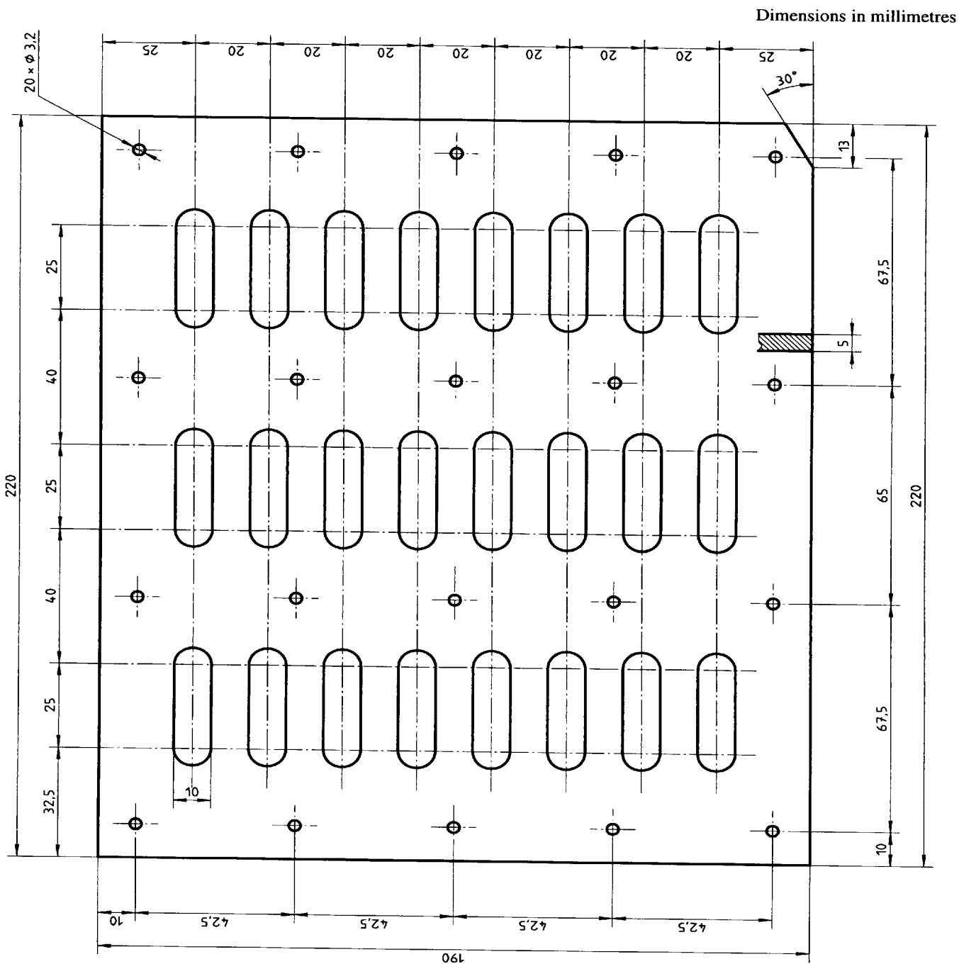
Figure 6 — Securing plate
