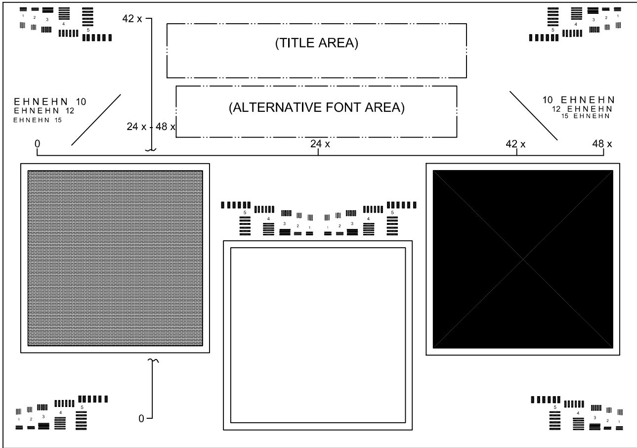
Figure 3 — Sample layout of Target 2
