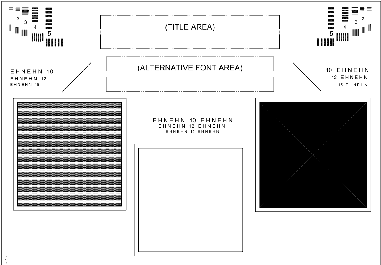
Figure 2 — Sample layout of Target 1
