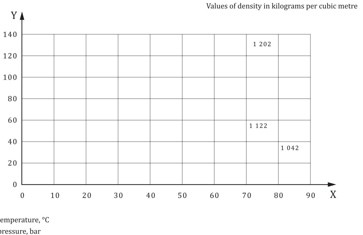
Figure 1 — Temperature/pressure graph for HFC 236fa pressurized with nitrogen to 25 bar at 22 \text{ }^\circ\text{C}
