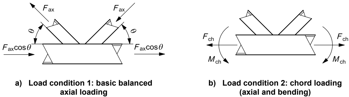
Figure E.3 — Load conditions for uniplanar RHS K-joints with gap
