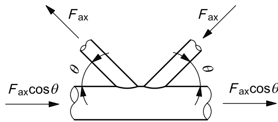
a) Load condition 1: basic balanced axial loading
