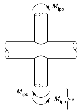
b) Load condition 2: in-plane bending
