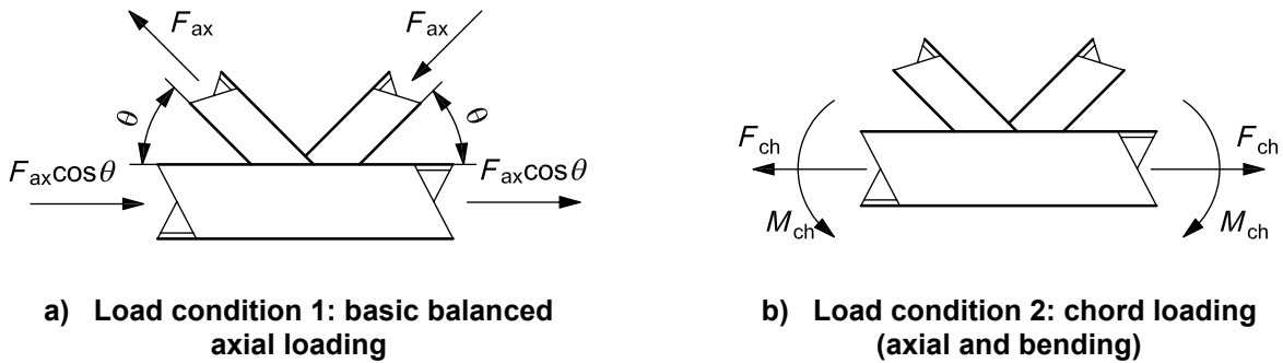
Figure E.12 — Load conditions for uniplanar RHS K-joints with overlap
