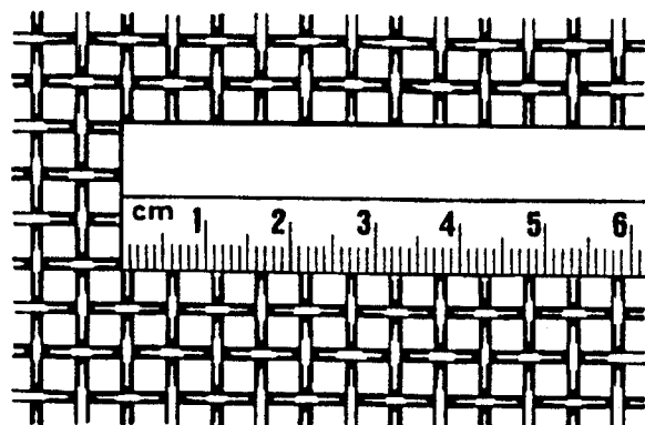
Figure 7 — Measured row with 10 pitches and 52,5 mm length
