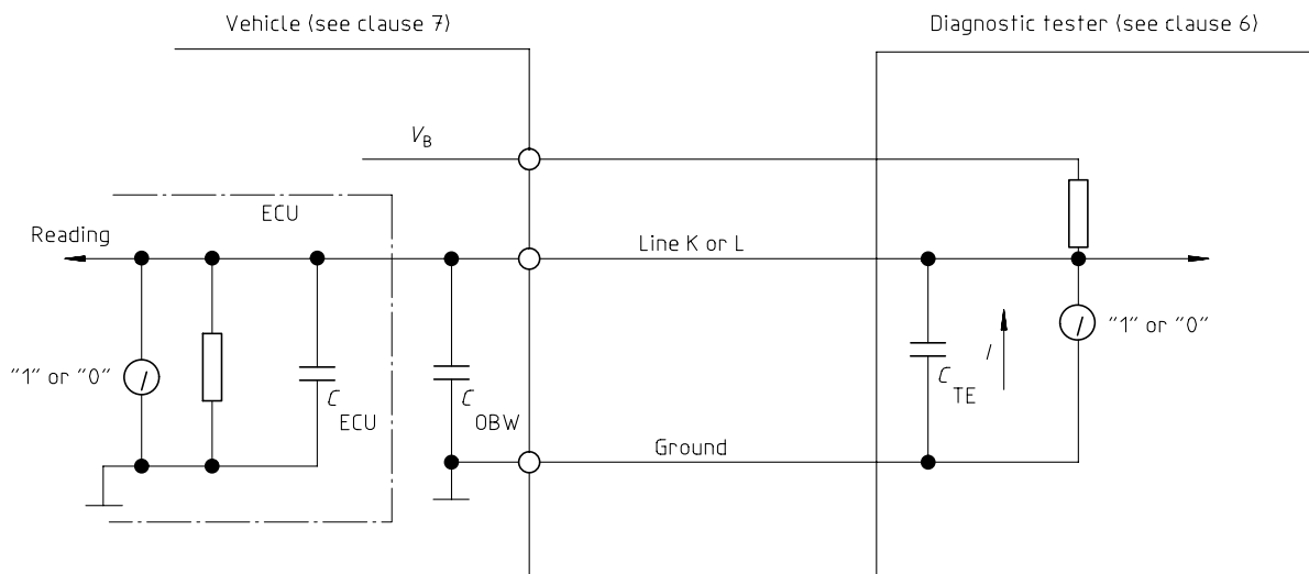
Figure 3 — Communication schematic
