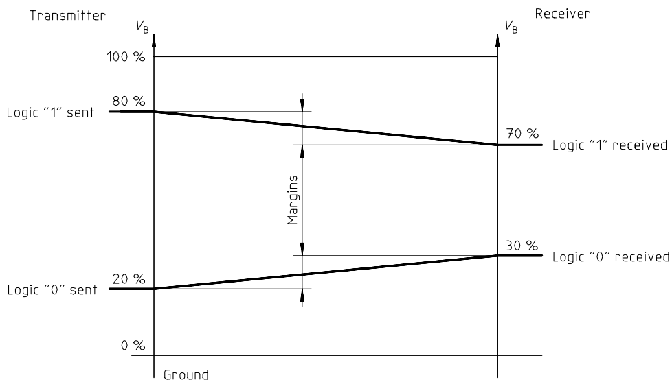
Figure 2 — Signal voltage levels, worst case values
