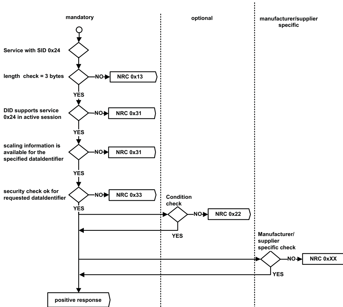
Figure 17 — NRC handling for ReadScalingDataByIdentifier service
