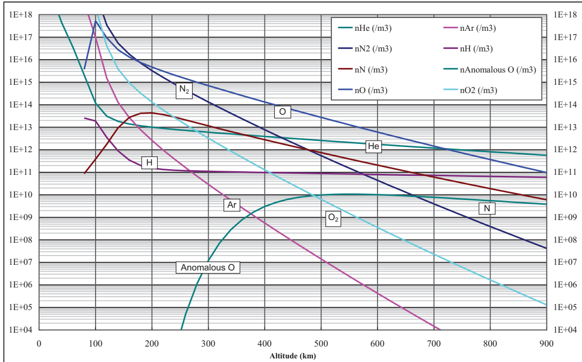
Figure A.3 — NRLMSISE00 mean concentration of atmosphere constituents for moderate solar and geomagnetic activity
