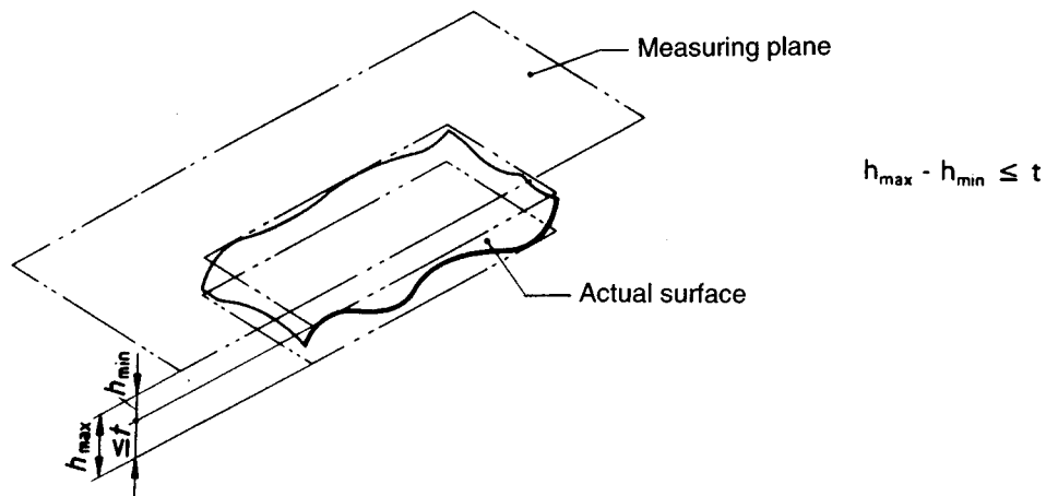
Figure 7: Flatness test
