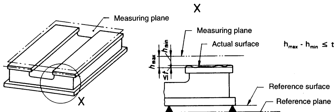
Figure 8: Parallelism test
