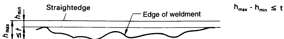
Figure 6: Straightness test
