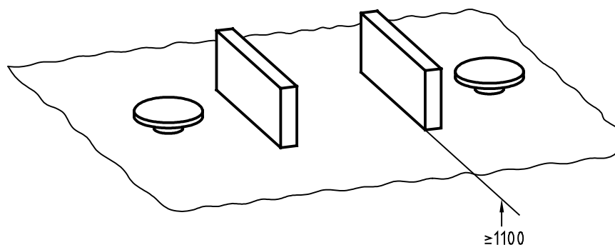
Figure A.11 — Prevention of defeat by position
