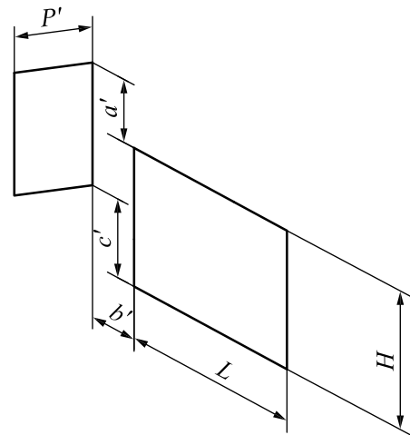
Figure C.3 — Side fin, main dimensions
