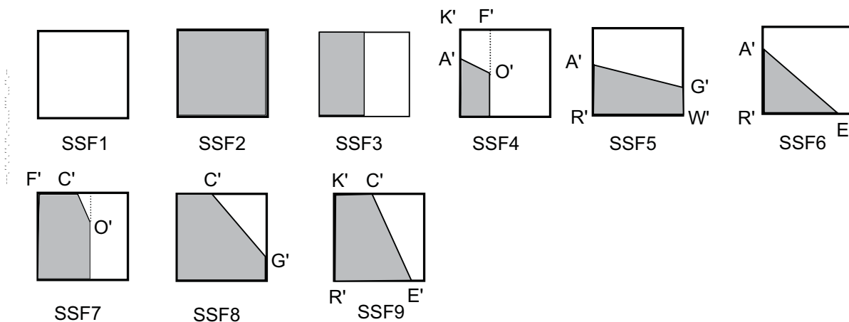
Figure C.6 — Shadow shapes of side fins
