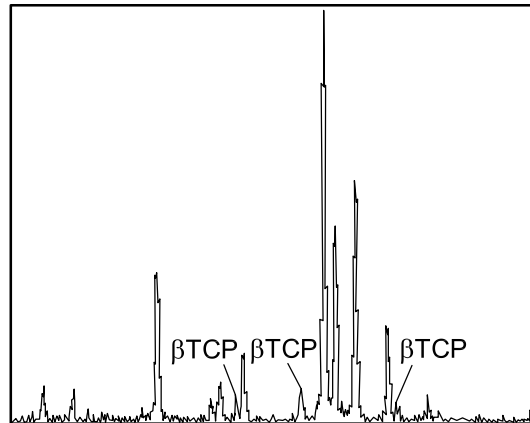
Figure C.3 — Mixture of hydroxyapatite and 5 % TCP
