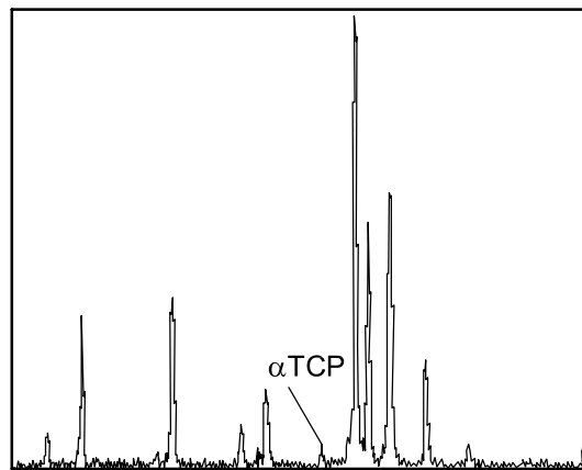
Figure C.4 — Mixture of hydroxyapatite and \alpha -tricalcium phosphate ( \alpha -TCP) at 5 % of mass
