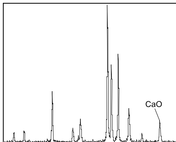
Figure C.5 — Mixture of hydroxyapatite and 5 % CaO
