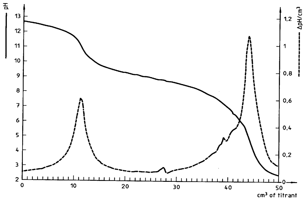
Figure B.1 – Example of titration and derivative curves
