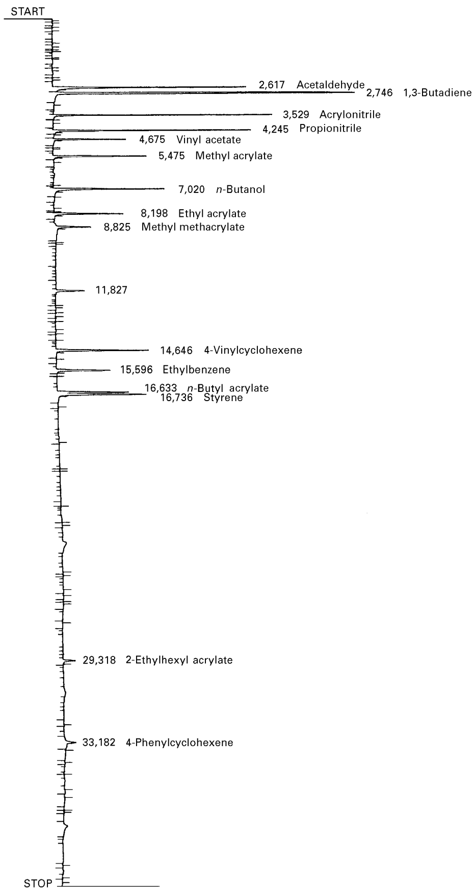
Figure 1 — Typical chromatogram
