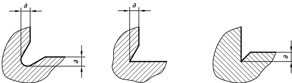
Figure 4 — Examples of undercut at an external edge
