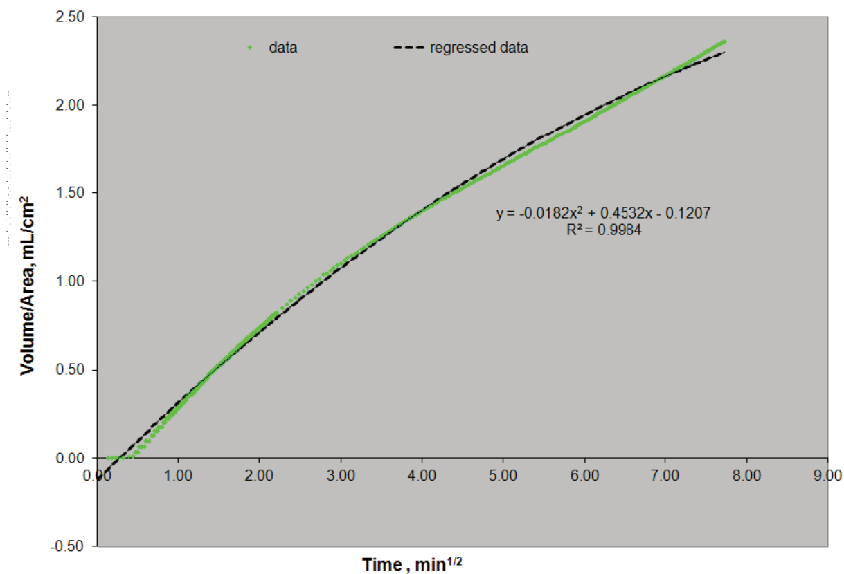
Figure 3 — Dynamic fluid loss example — 4,2 kg/m 3 CMHPG (35 lb/Mgal) at 82 °C (180 °F), 6 900 kPa (1 000 psi)
