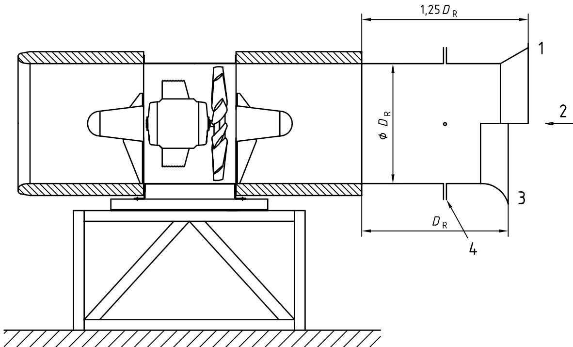
Figure 11 — Flow-measuring installation (upstream Pitot traverse)
