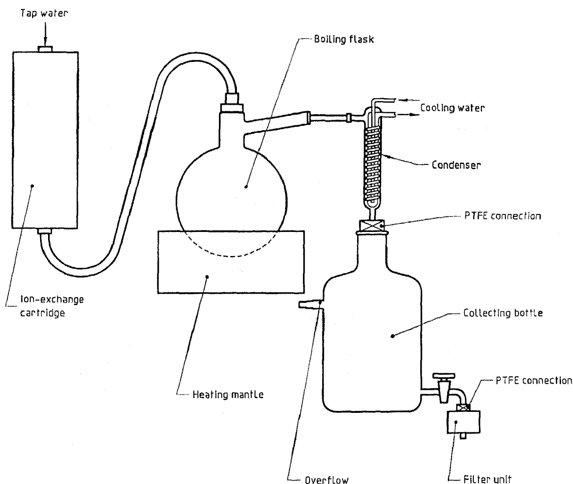
Figure E.3 — Water purification: deionization, distillation, filtration
