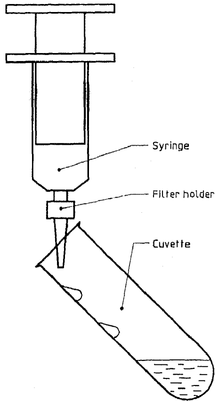
Figure E.1 — Solvent filtration, small quantities
