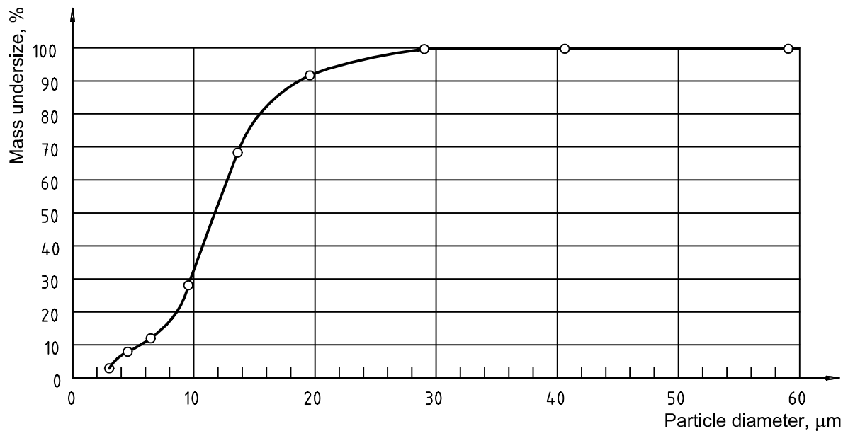
Figure A.1 — Cumulative mass percentage undersize by Andreasen pipette
