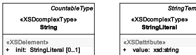
Figure 75 — Declaration and Initialisation of a string
