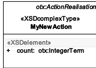
Figure D.4 — Reusing an OTX Core type in a new ActionRealisation
