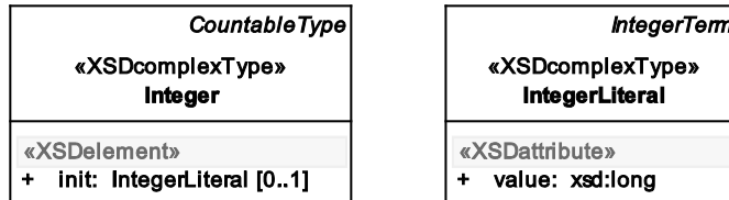
Figure 74 — Declaration and Initialisation of an Integer
