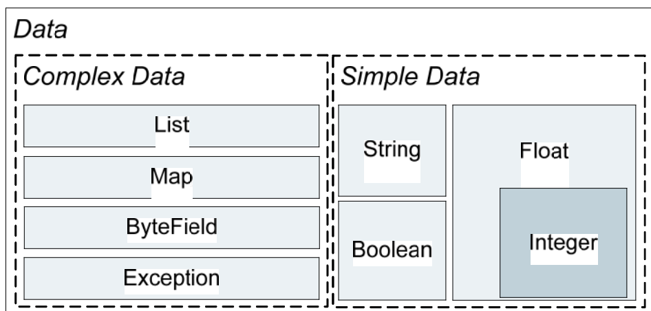
Figure A.4 — Nesting of data type value spaces
