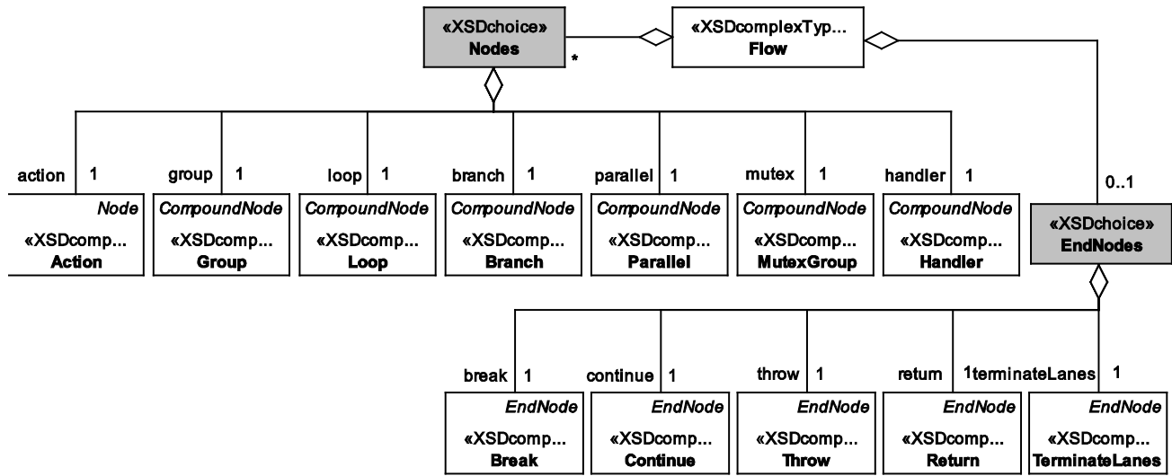
Figure 81 — Data model view: Flow
