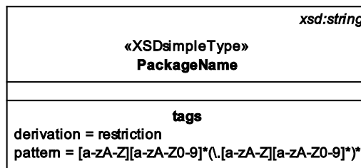
Figure 64 — Data model view: PackageName
