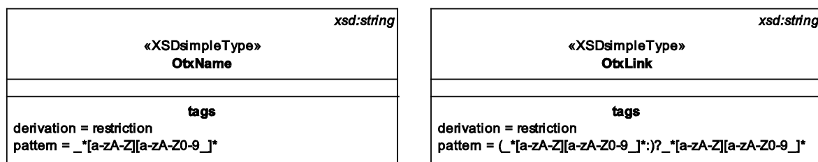
Figure 65 — Data model view: OtxName and OtxLink
