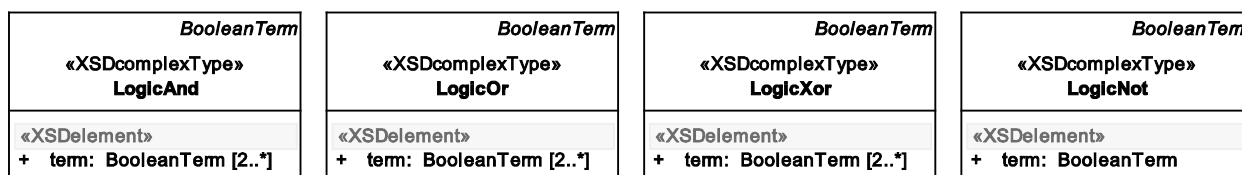
Figure 56 — Data model view: Logic operations
