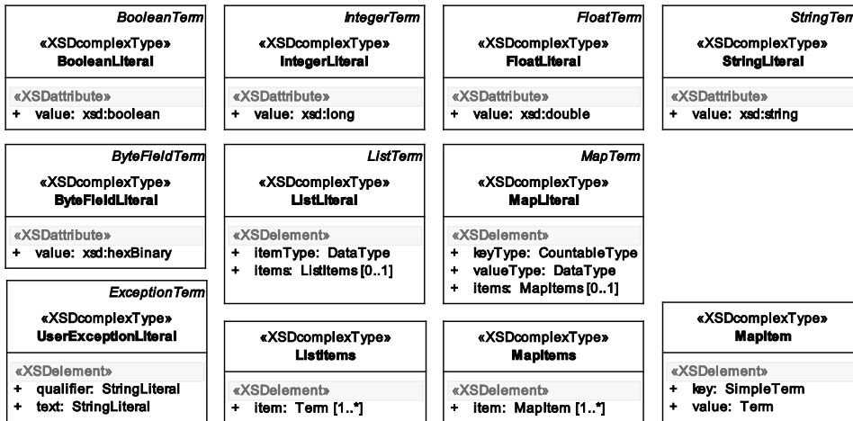
Figure 51 — Data model view: Literal terms
