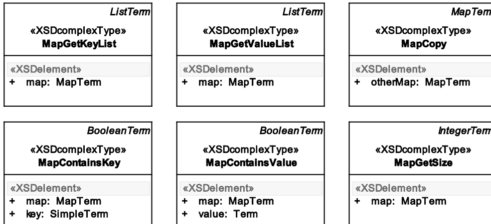
Figure 61 — Data model view: Map related terms
