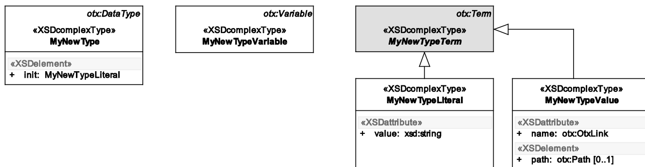
Figure D.2 — Deriving new data types and terms
