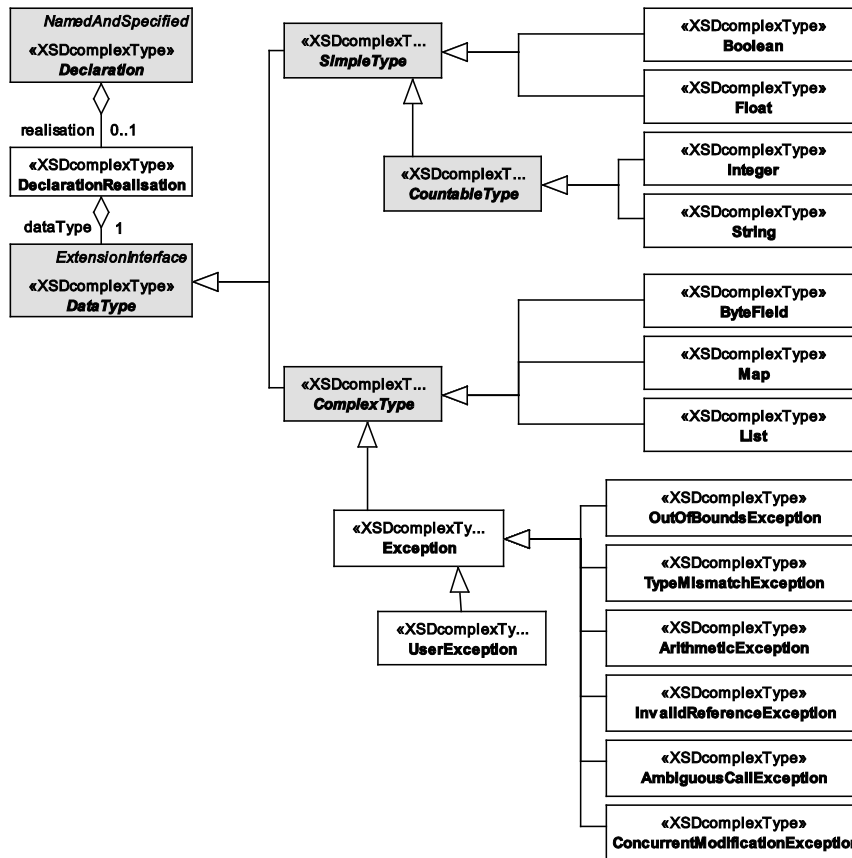
Figure 71 — Overview: Data type hierarchy in declaration blocks
