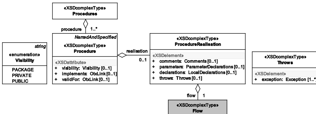
Figure 18 — Data model view: Procedures
