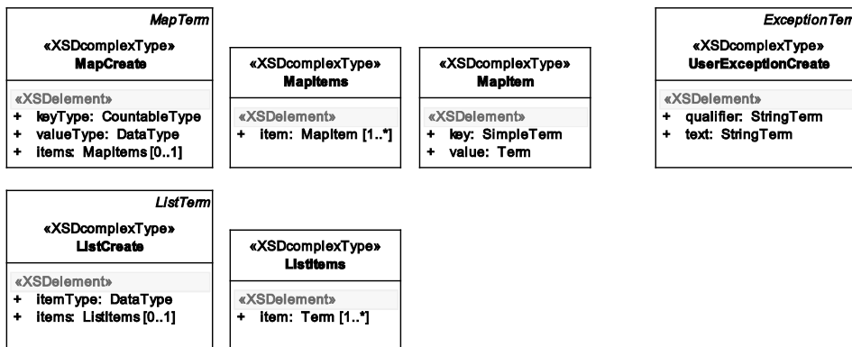
Figure 53 — Data model view: Creation terms
