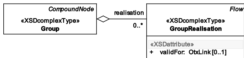
Figure 25 — Data model view: Group
