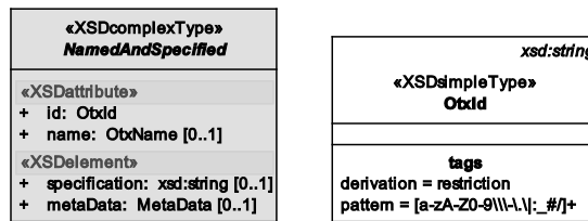
Figure 66 — Data model view: NamedAndSpecified
