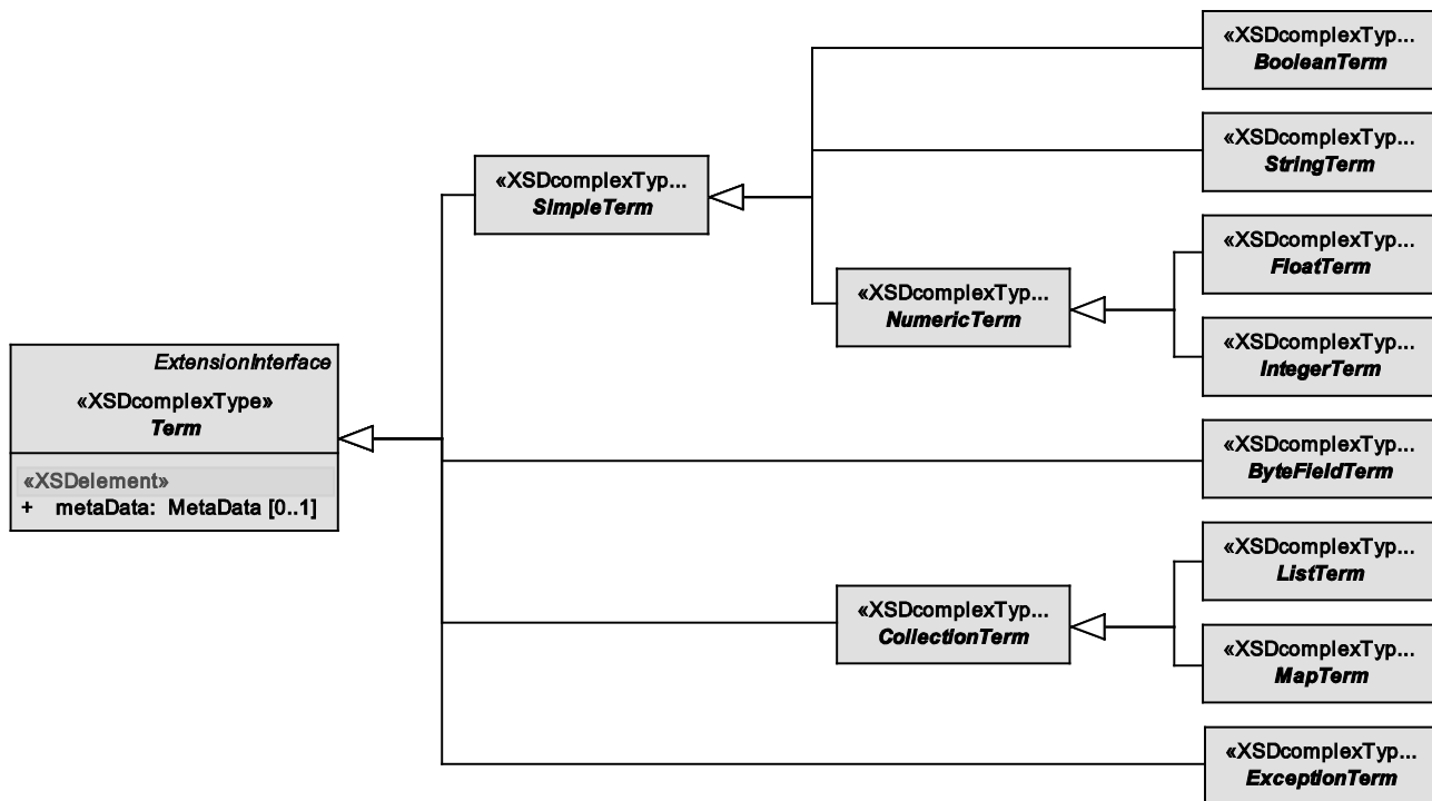
Figure 50 — Data model view: Term hierarchy
