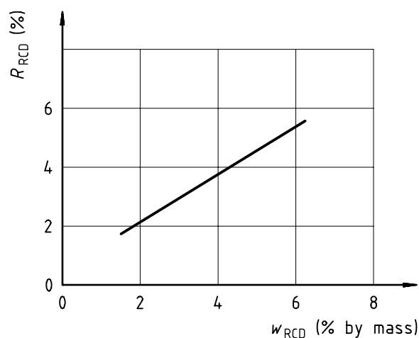
b) Estimated reproducibility R_{RCD} as a function of w_{RCD} (reactivity-to- CO_2 parameter for dust)
