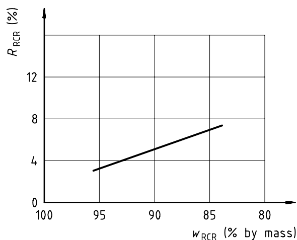
a) Estimated reproducibility R_{RCR} as a function of w_{RCR} (reactivity-to- CO_2 parameter for residue)
