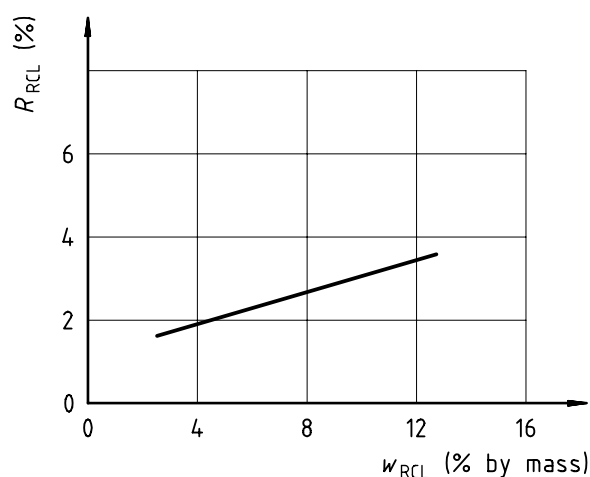
c) Estimated reproducibility R_{RCL} as a function of w_{RCL} (reactivity-to- CO_2 parameter for loss)
