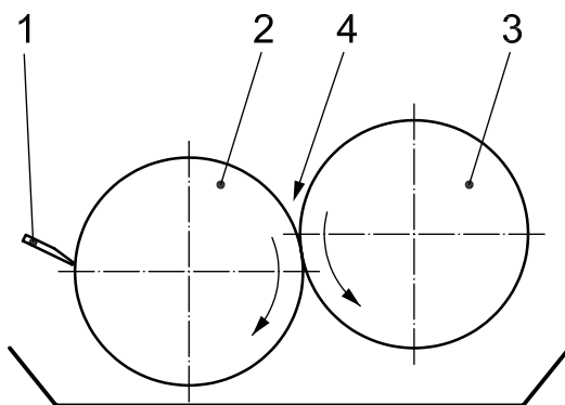
Figure 27 — Roller gluing unit with dosing roller
