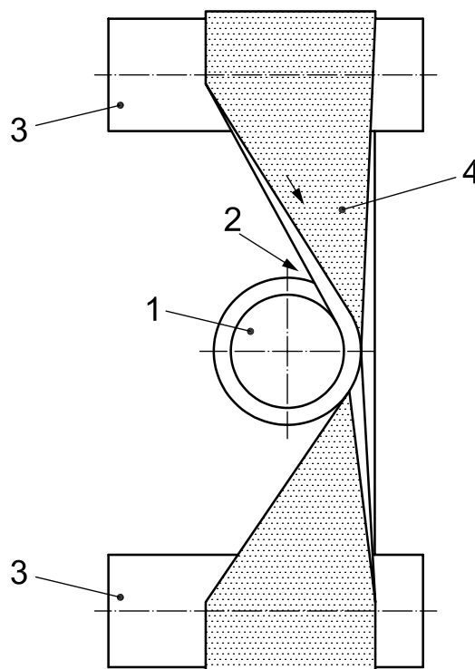
Figure 25 — Winding belt in-running nip on tube winding machine (view of drive drums)
