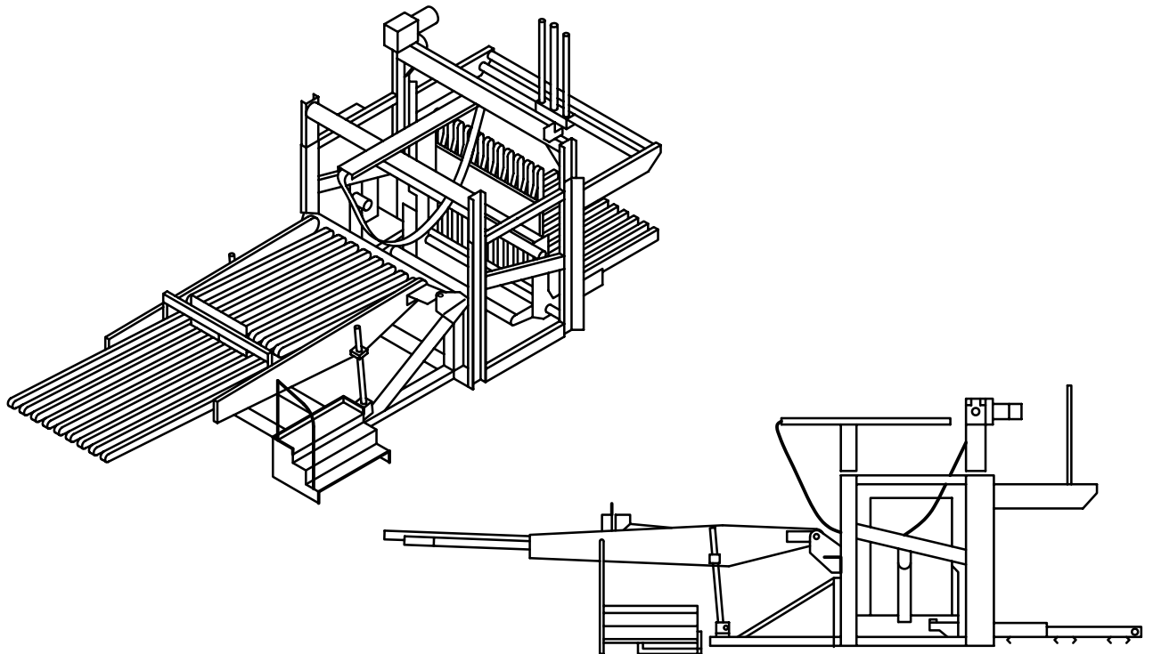
Figure 21 — Pre-feeder with pile turner
