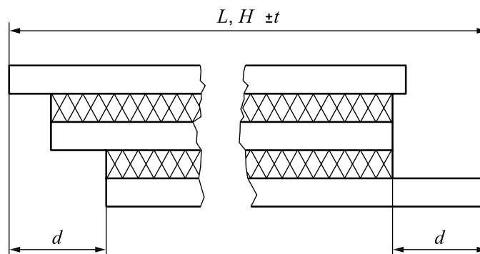
Figure 2 — Displacement
