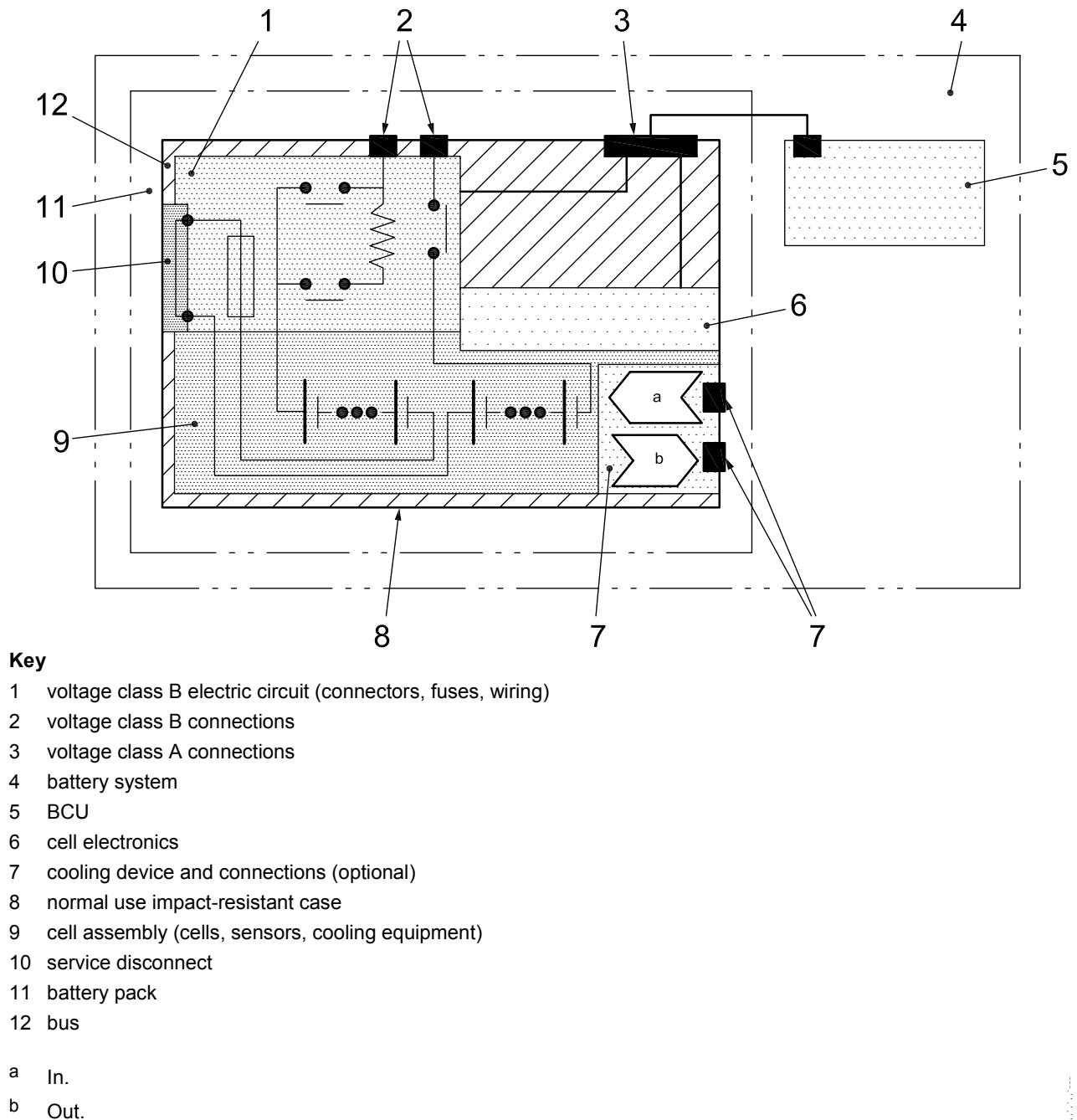
Figure A.3 — Typical configuration of a battery system with external BCU
