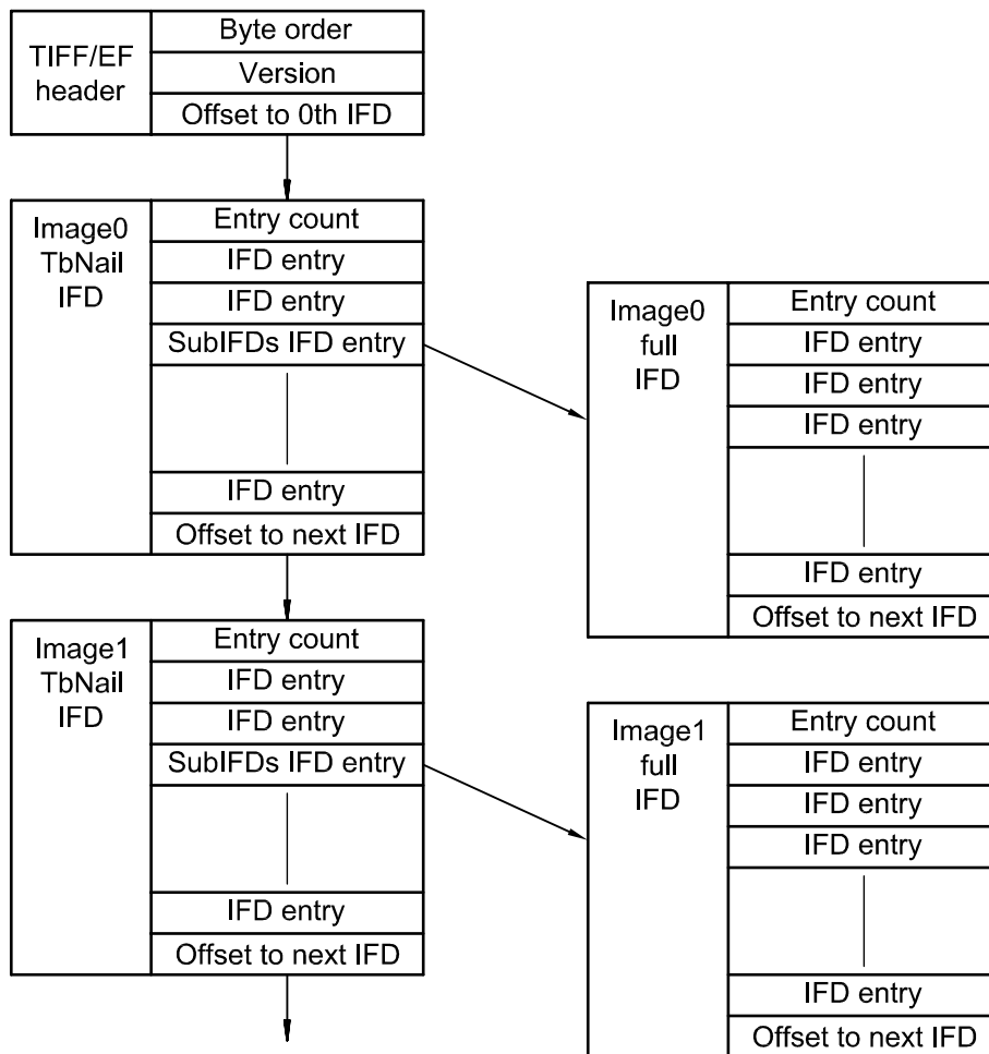
Figure 3 — TIFF/EP encoding structure with image chaining
